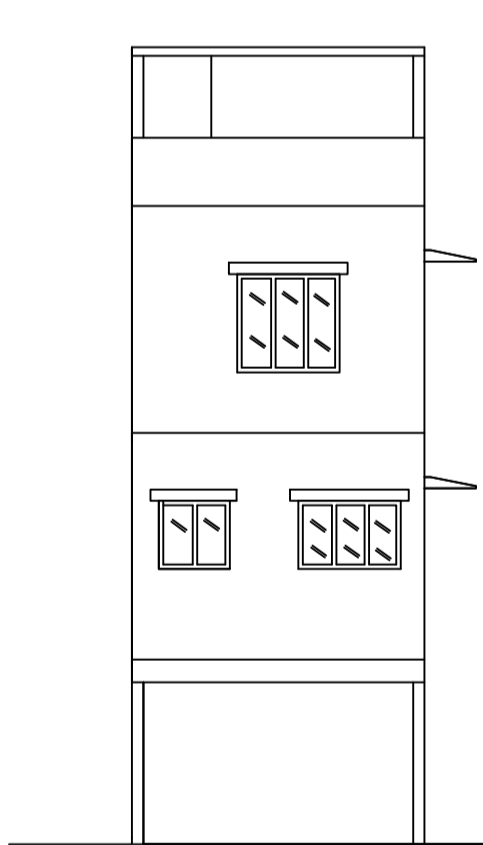
FRONT ELEVATION
